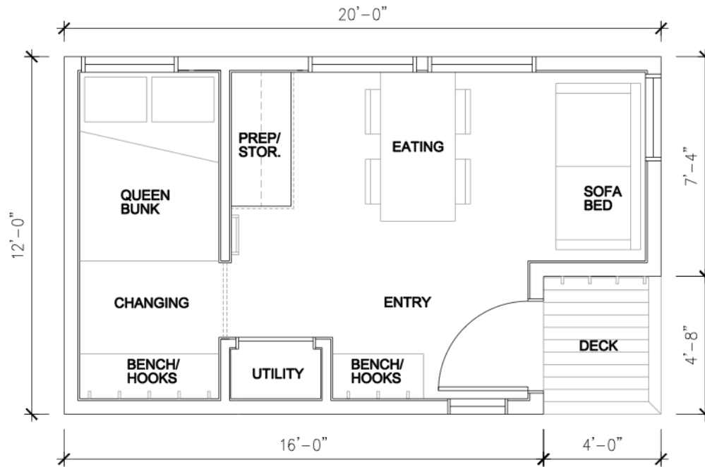
MAIN LEVEL
